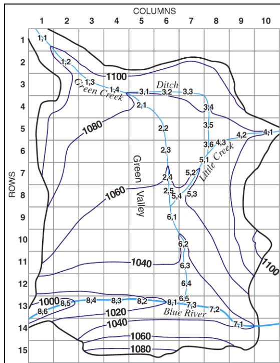
Figure 1. An SFR1 stream network. (Prudic et. al. 2004).
